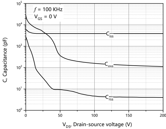
Figure 3. Typ. capacitances
