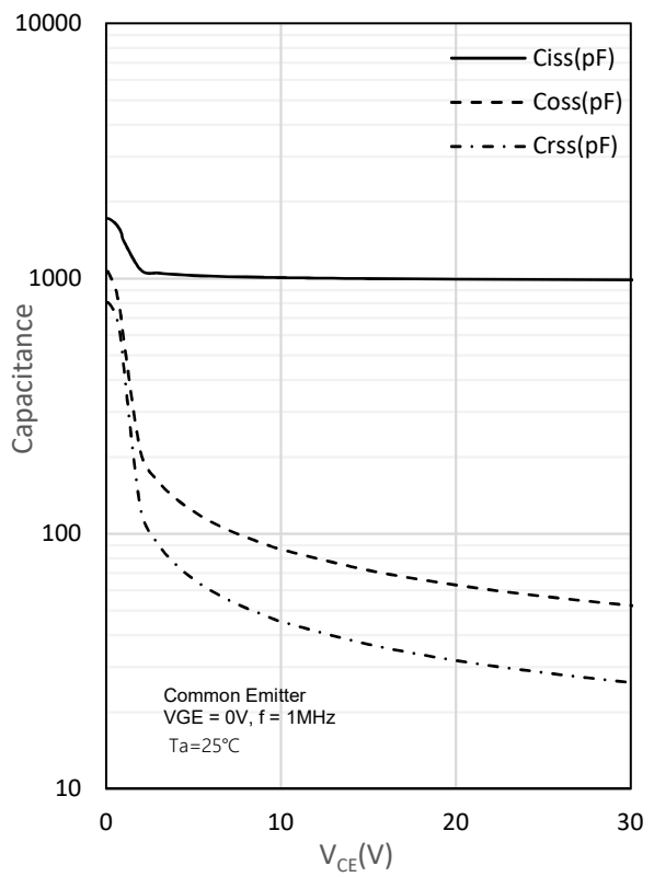
Fig. 12 Capacitance characteristics
